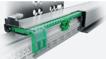
Effortless opening, excellent running characteristics and complete synchronisation.
