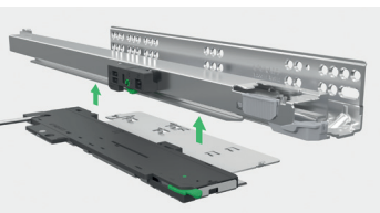
Tool-free installation and removal directly on the slide.
